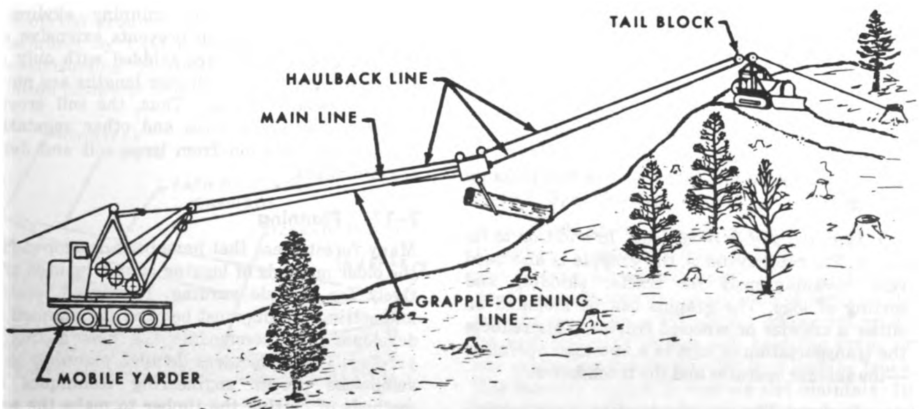
Figure 7-25. Typical three-line running skyline rigged for grapple yarding.
